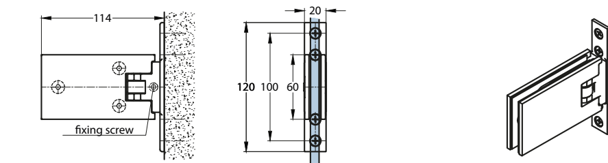
for all-glass showers according to EN 14428 with sealing profiles
