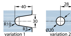
glass cut-out
