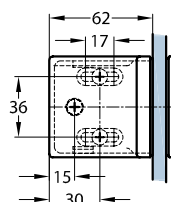
for 8 mm glass
