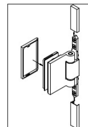
glass cut-out
