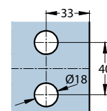
glass cut-out
